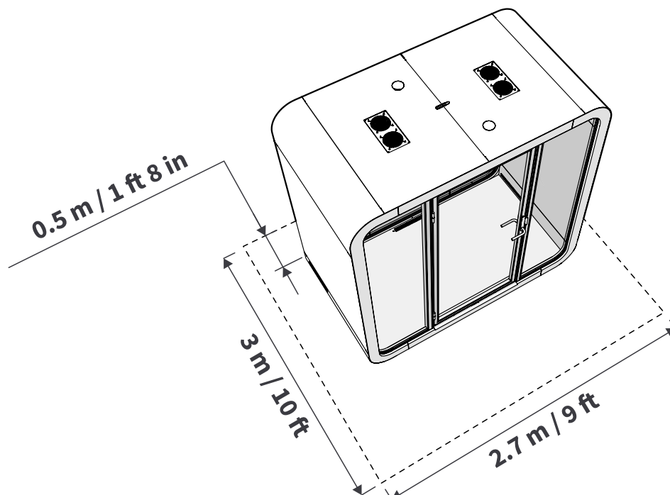
Figure 3: Installation space measurements
