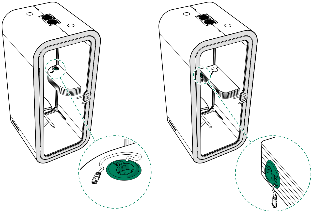
Figure 1: Power outlet in Framery O and Framery O with wide table
