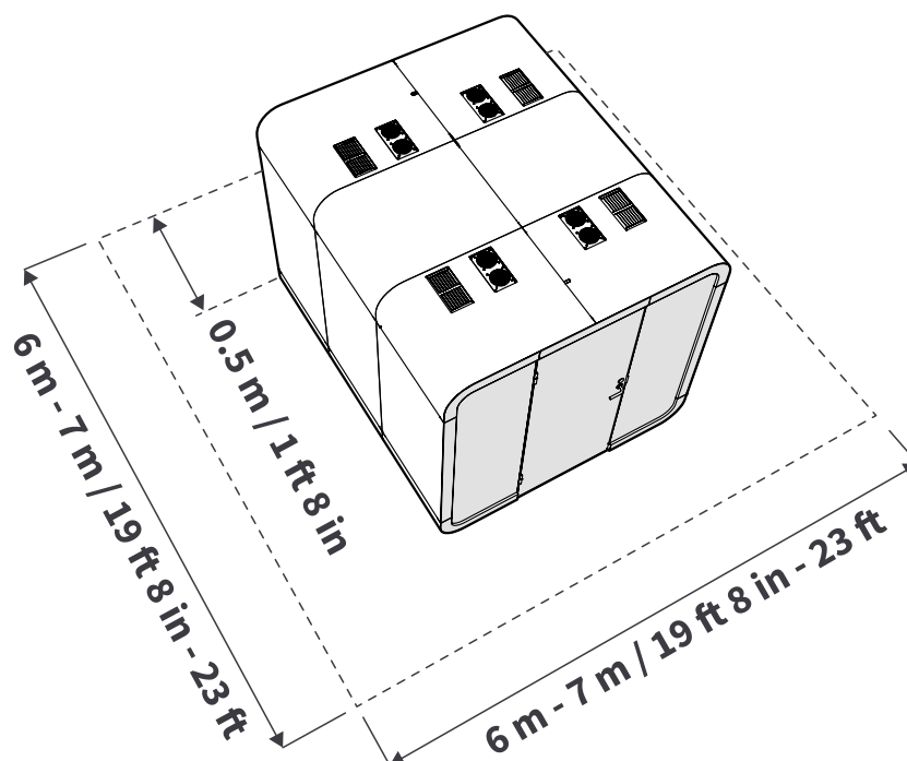
Figure 3: Installation space measurements of the 2Q pod
