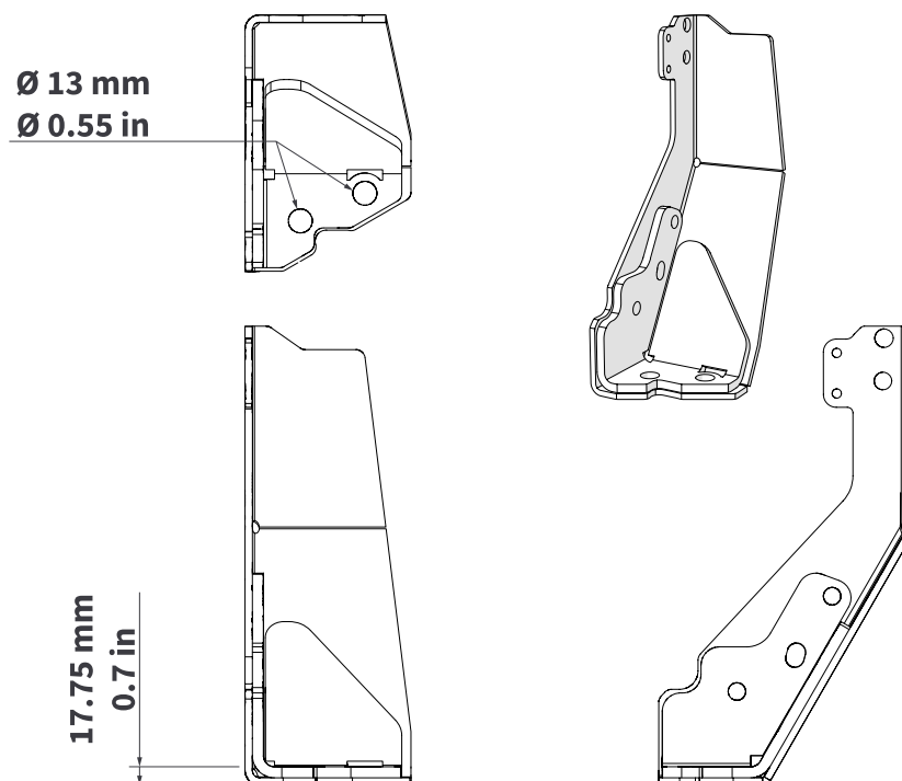
Figure 2: Framery Four seismic kit
