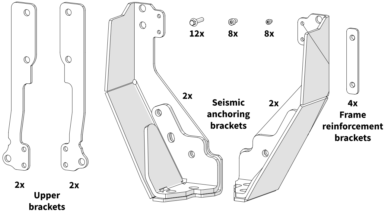
Figure 2: Framery Four seismic kit
