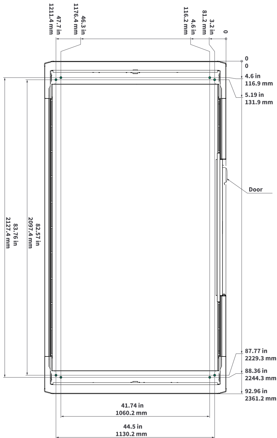
Figure 1: Framery Four seismic anchoring dimensions
